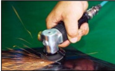
▲ Grinding Operation
