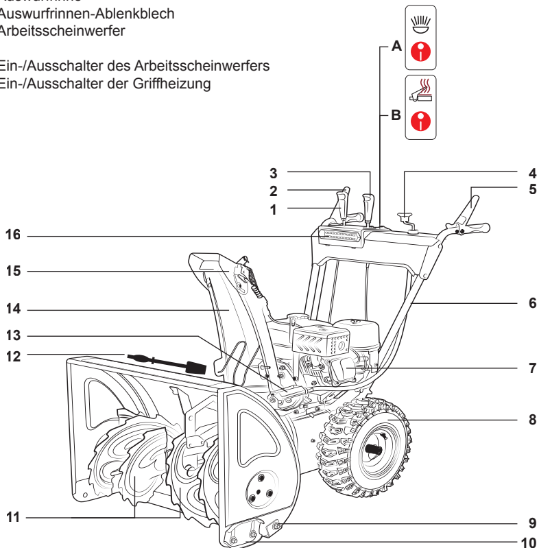
Modell SFR-65
